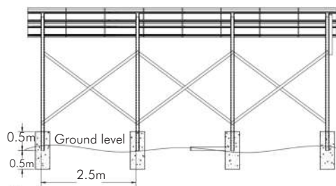
Steel Section Detail
