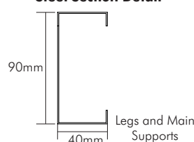
Steel Section Detail
