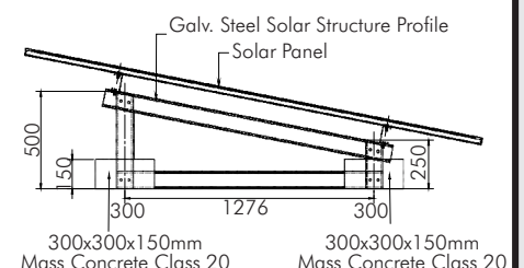
Concrete Mount Schematic
