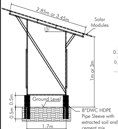
Ground Mount Support Schematic
