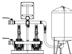
TWO PUMP SINGLE OR PARALLEL OPERATION
