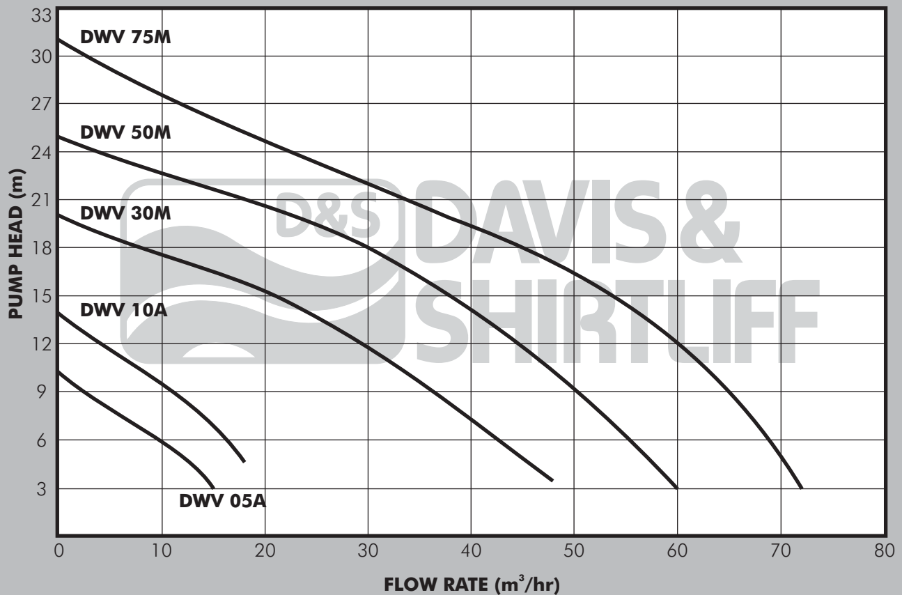
DWV 30M/50M/75M
