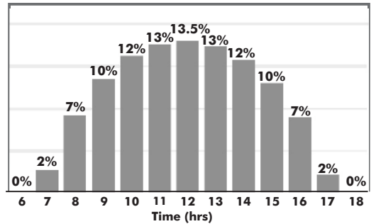
% Daily Output Graph 2
