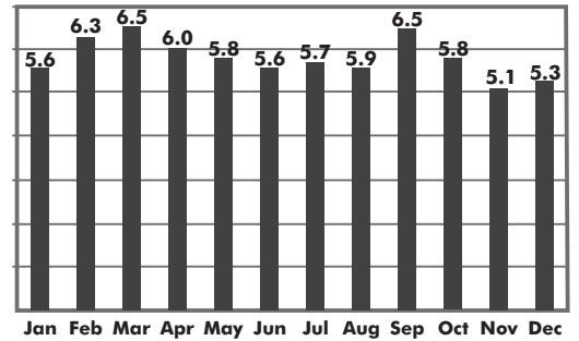
Average Daily Irradiation Values (Kwhr/m 2 ) Graph 1
