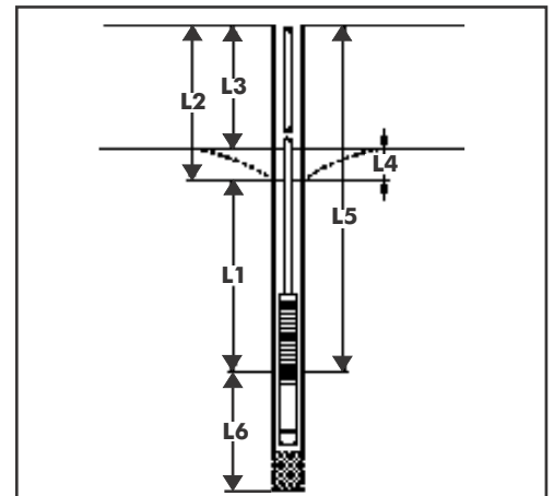
Fig. 4 Borehole Measurements
